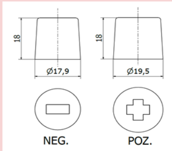
Terminal type
