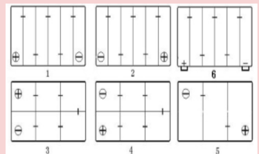
Terminal layout
